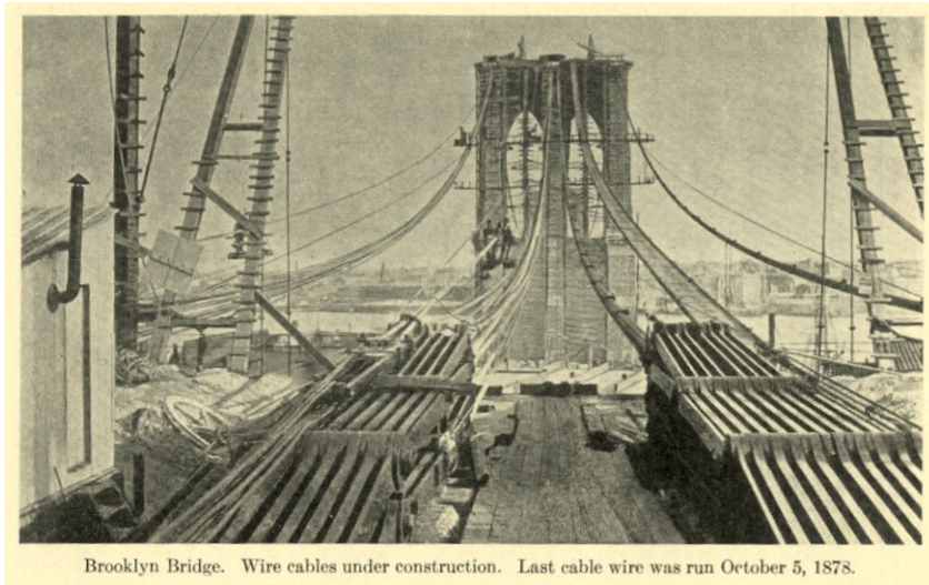
Brooklyn Bridge. Wire cables under construction. Last cable wire was run October 5, 1878.
